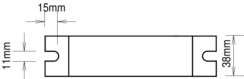
MOUNTING FOOT DETAIL
