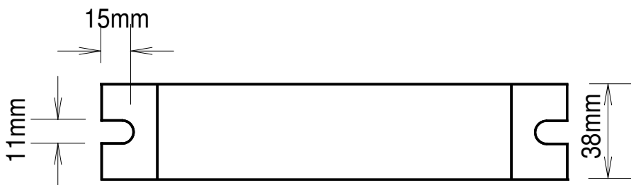
MOUNTING FOOT DETAIL
