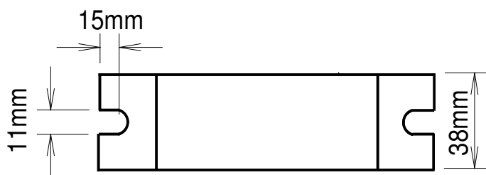
MOUNTING FOOT DETAIL
